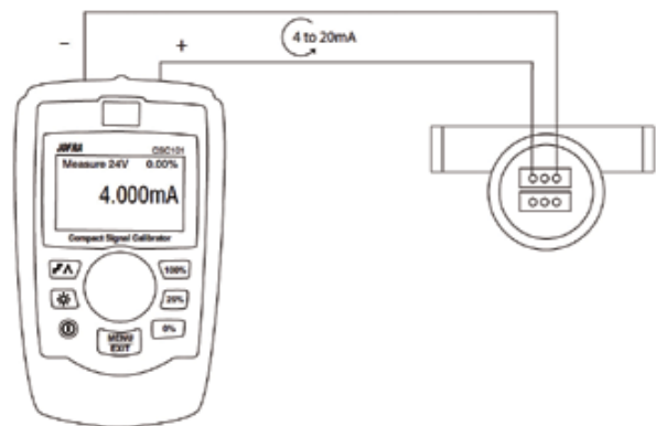
Measure mA, CSC 101 supplying 24 VDC
