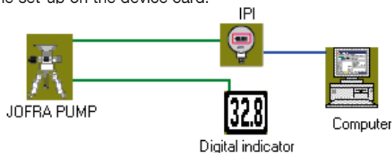
Set-up with JOFRA DPC-500 system D and DPC-J reference sensor connected to a PC with JOFRACAL
